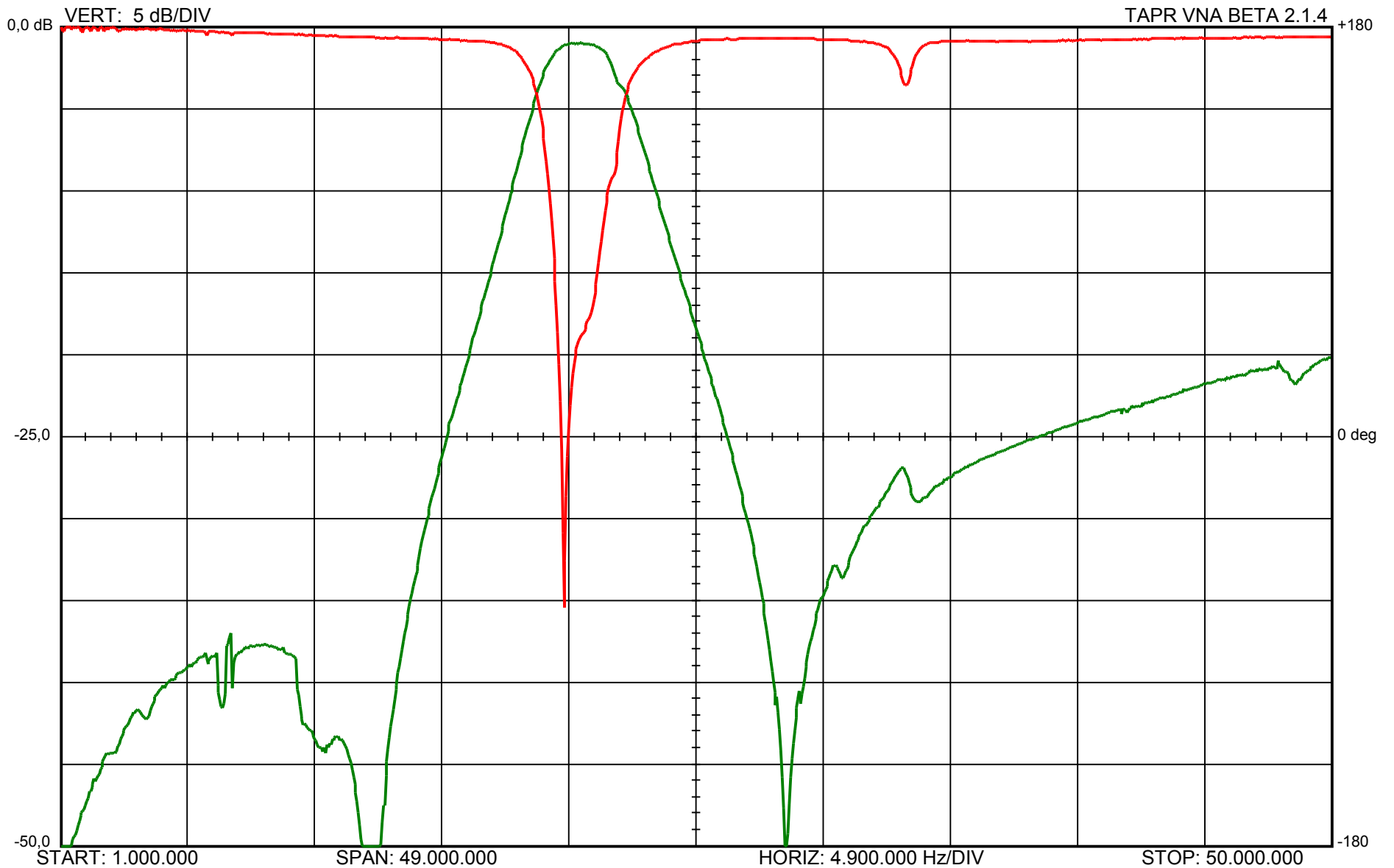
15m ICE Multiband Filter - EA4TX 23/Aug/08
