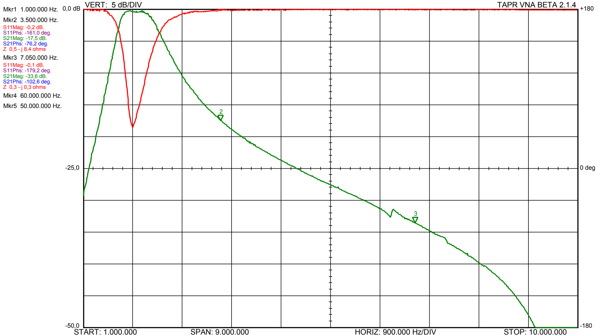
160m ICE Multiband Filter - EA4TX 23/Aug/08
