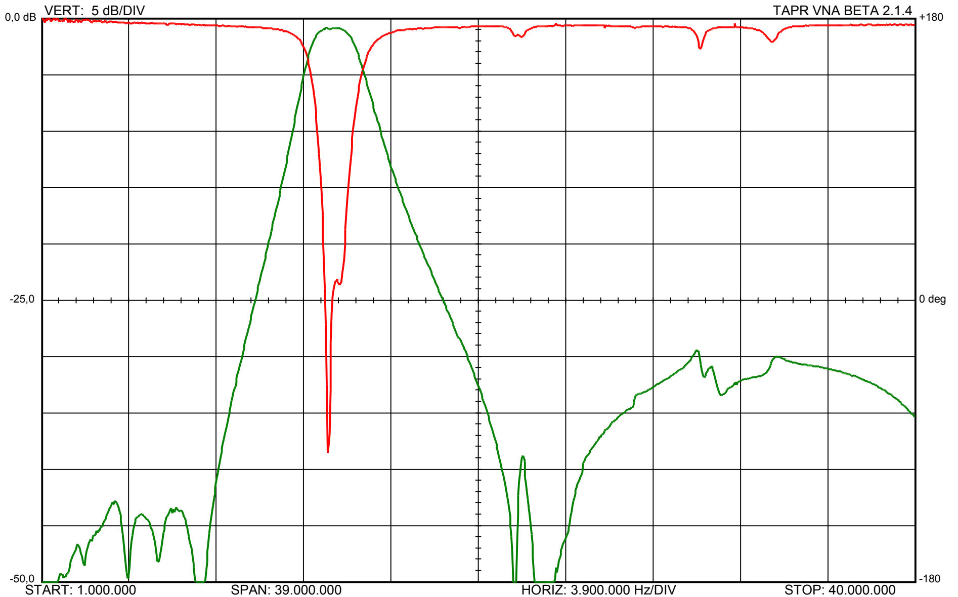
20m ICE Multiband Filter - EA4TX 23/Aug/08
