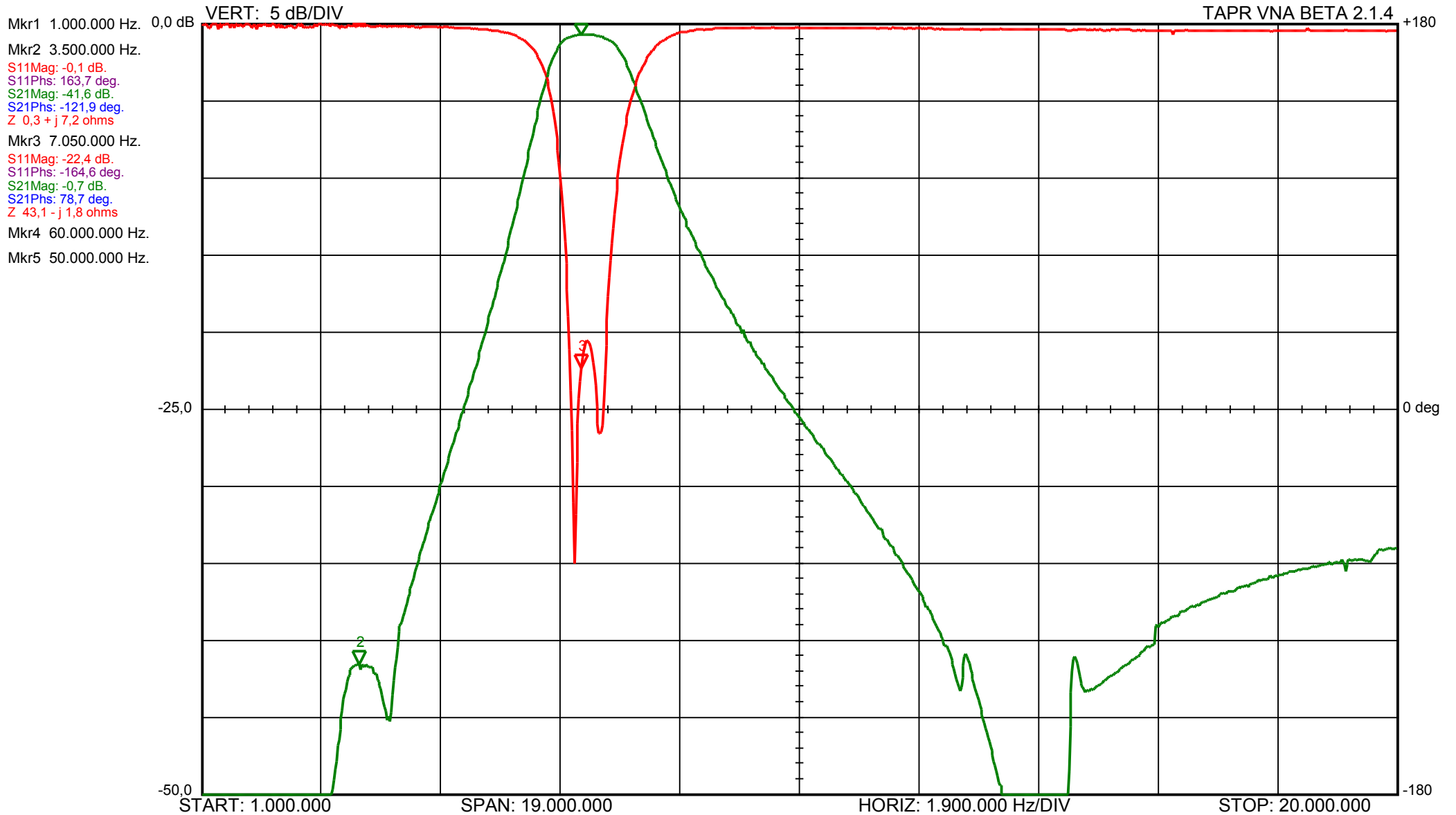
40m ICE Multiband Filter - EA4TX 23/Aug/08
