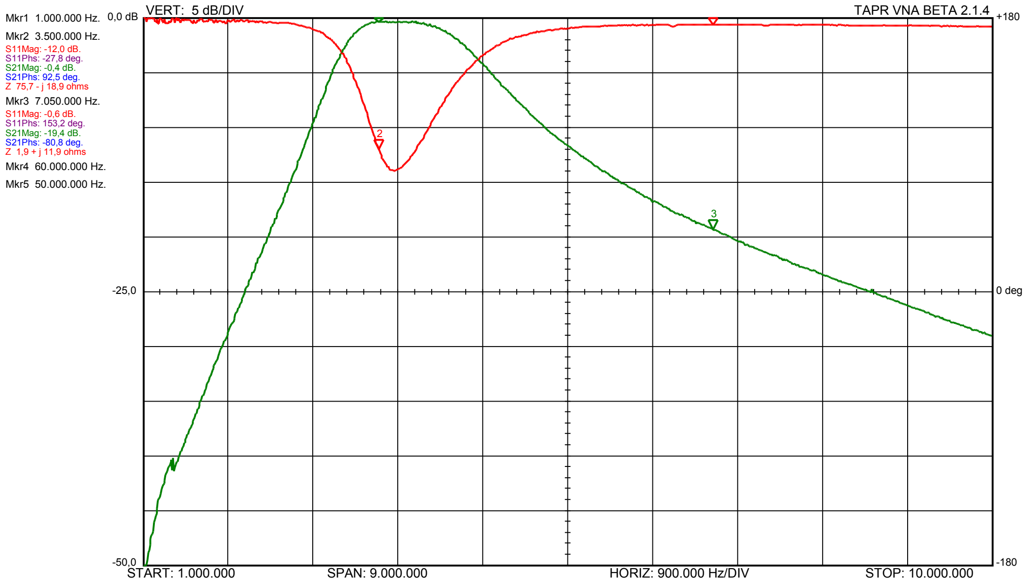
80m ICE Multiband Filter - EA4TX 23/Aug/08
