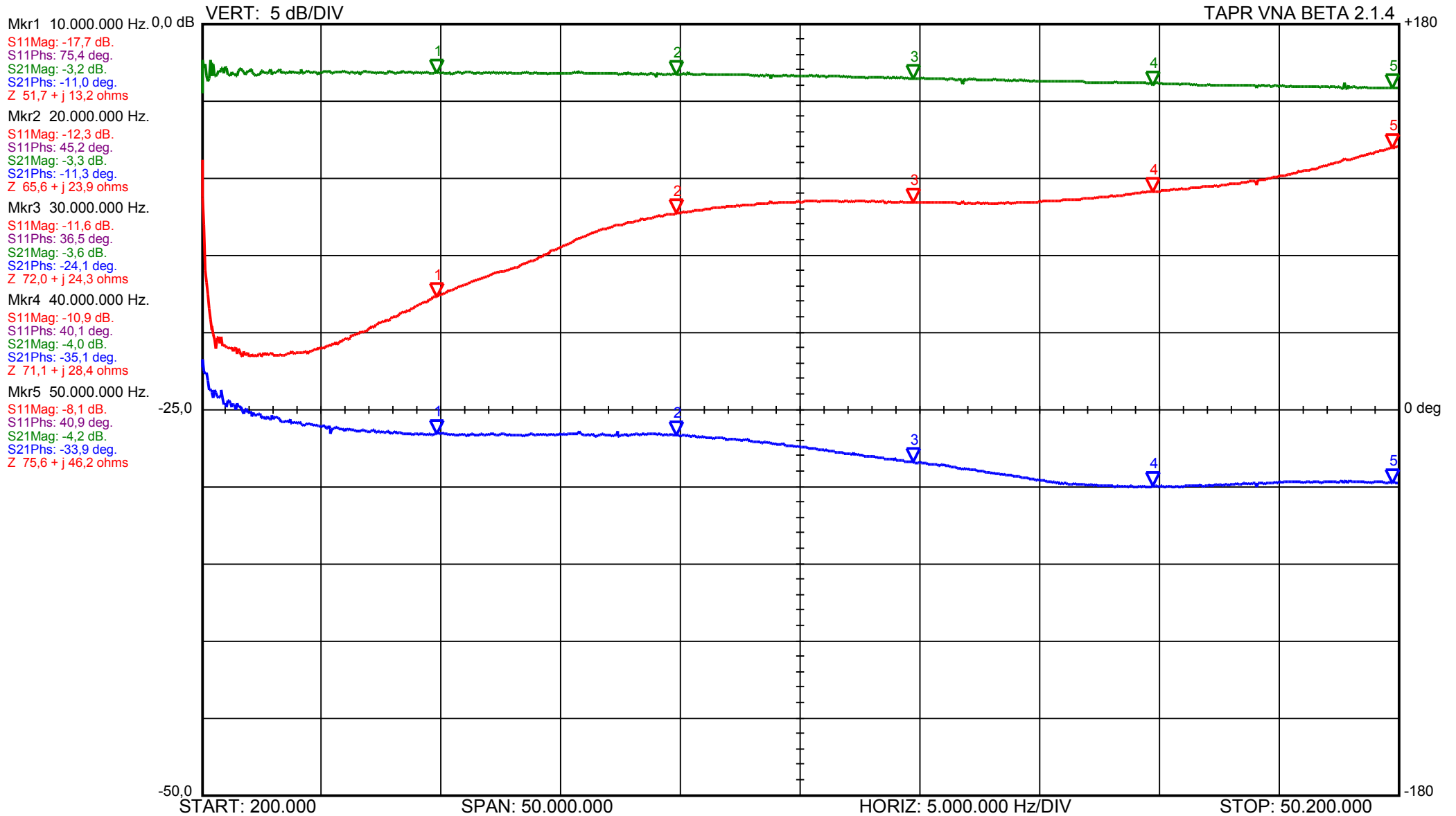
Measurement between Port 1 and Port 3 of a 0° - 180° Hybrid while Port 2 is terminated with 50 Ohm - DH1TW 20/Aug/2008
