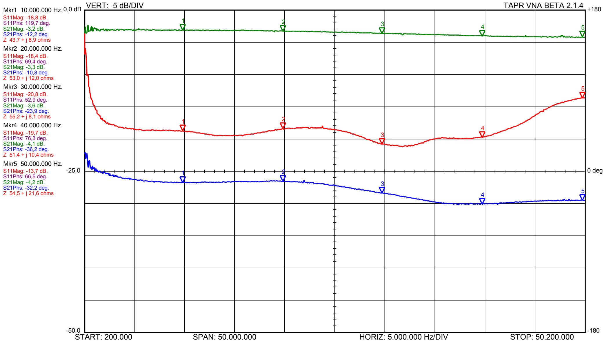
Measurement between Port 3 and Port 1 of a 0° - 180° Hybrid while Port 2 is terminated with 50 Ohm - DH1TW 20/Aug/2008
