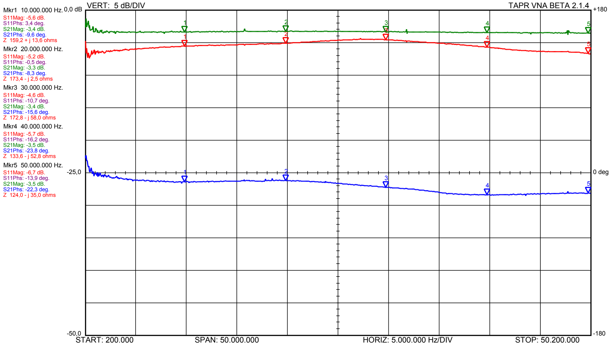
Measurement between Port 1 and Port 3 of a 0° - 180° Hybrid while Port 2 is open - DH1TW 20/Aug/2008
