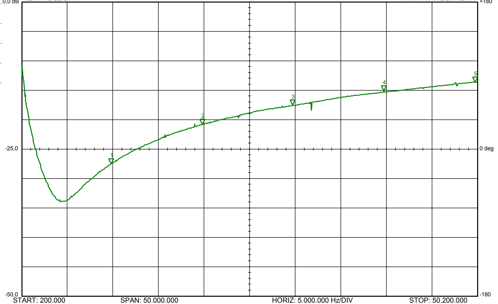
Measurement between Port 2 and Port 3 of a 0° - 180° Hybrid while Port 1 is terminated with 50 Ohm - DH1TW 20/Aug/2008
